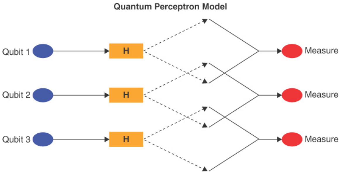
Figure 6-2 The Quantum Perceptron Model
