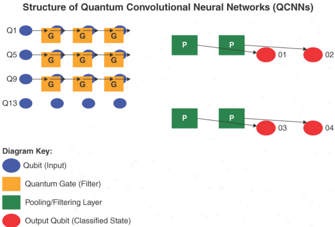
Figure 6-3 Quantum Convolutional Neural Networks (QCNNs)
