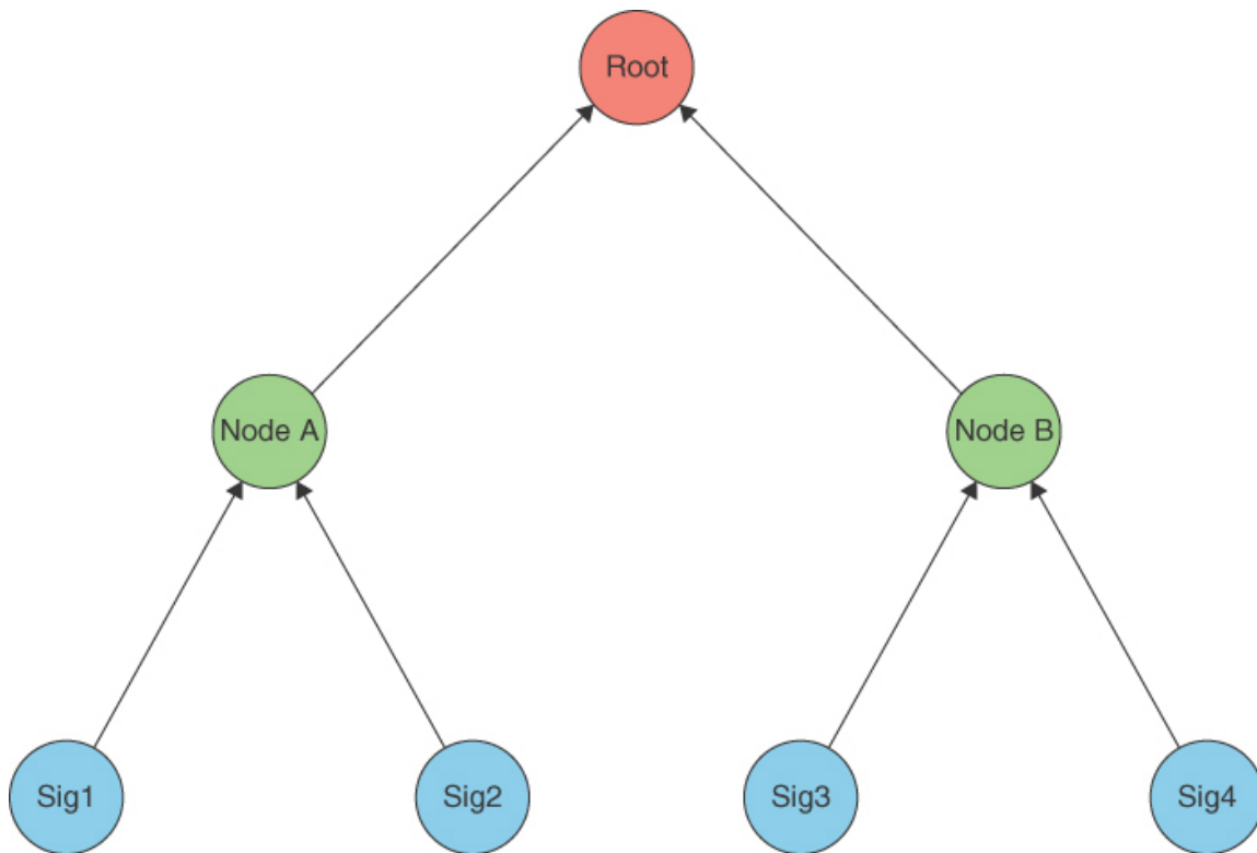
Figure 7-7 Merkle Signature Scheme
