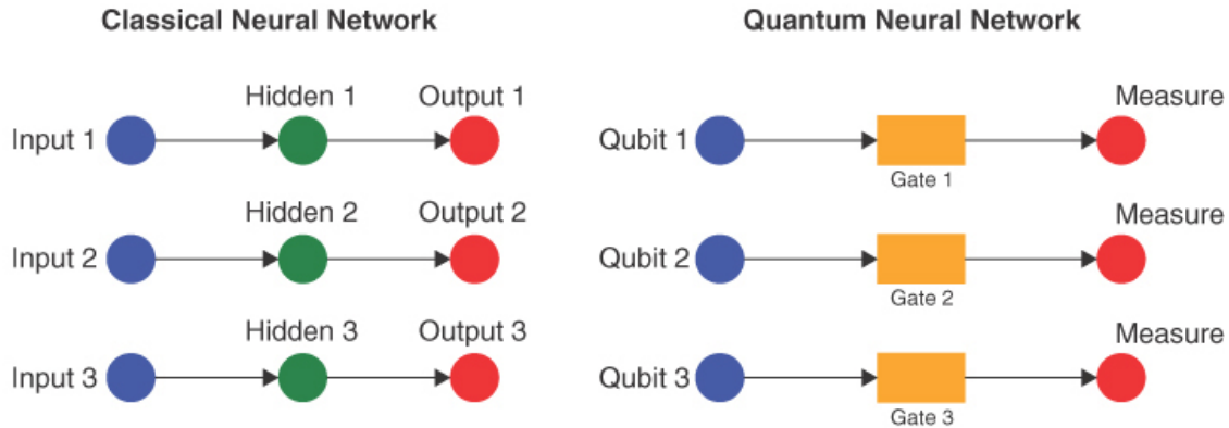
Figure 6-1 Classical vs. Quantum Neural Networks
