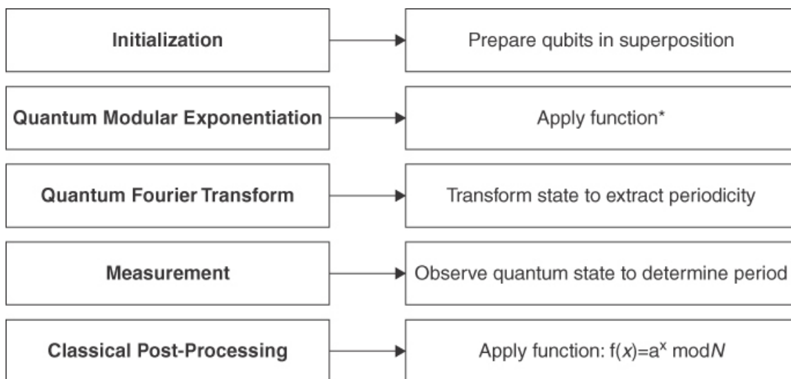
Figure 4-2 Steps of Shor's Algorithm
