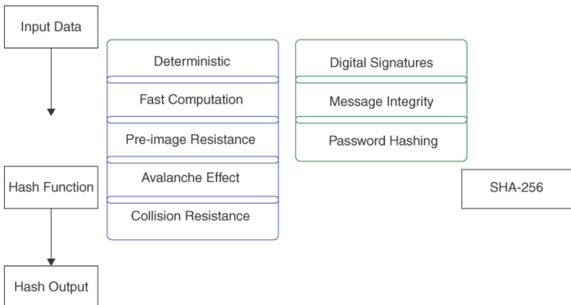
Figure 7-6 Key Concepts of Hash-Based Cryptography
